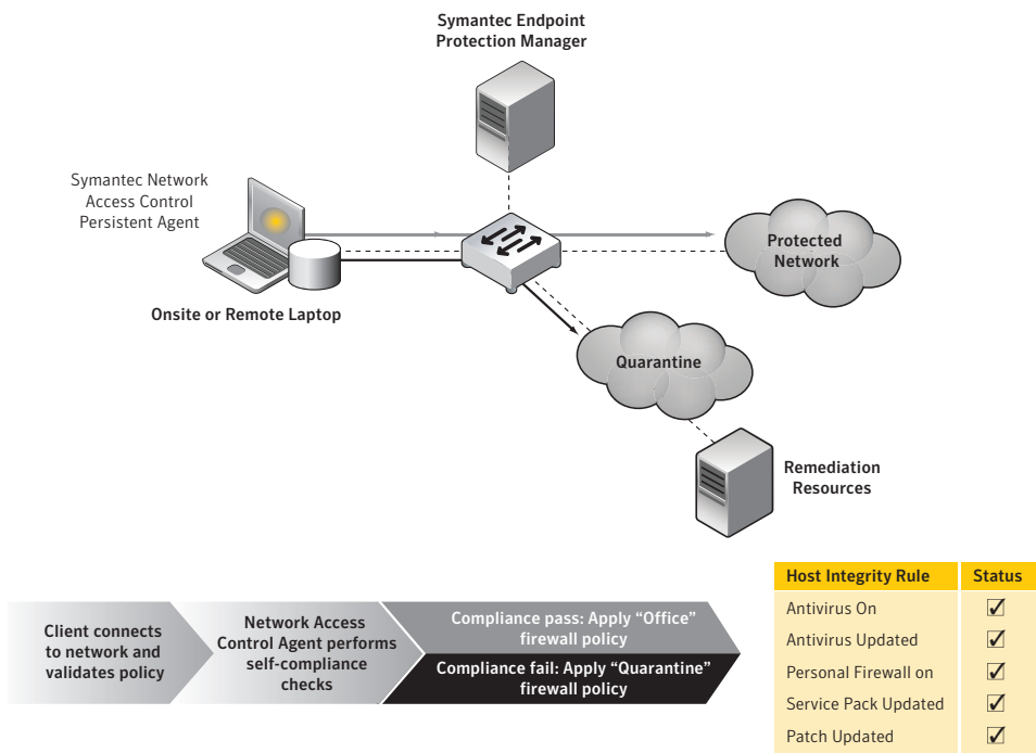
Figure 4. Persistent Agent
